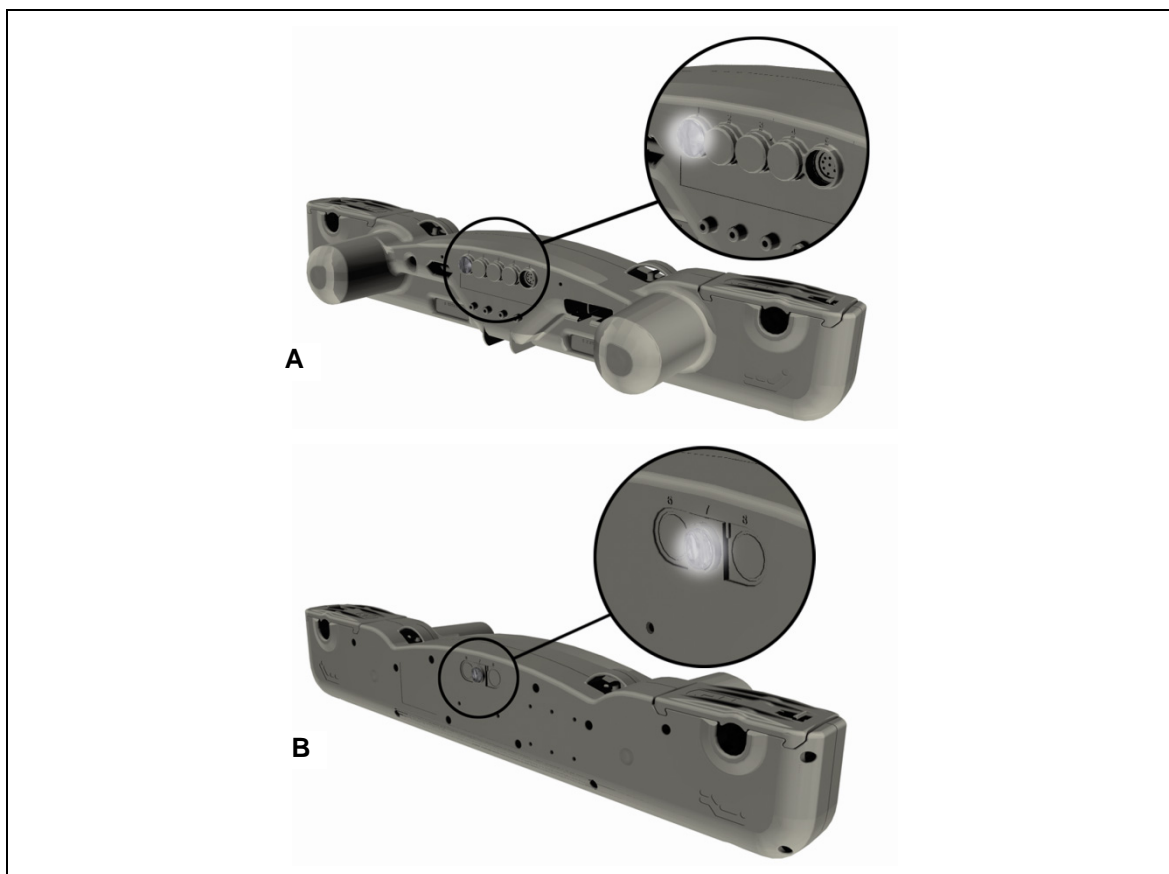
Figure 15 Location of the integrated floor lighting (optional)
