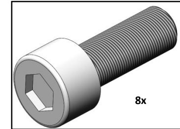
Zylinderkopfschraube M6x25mm SW5 cylinder head screw M6x25mm AF5
