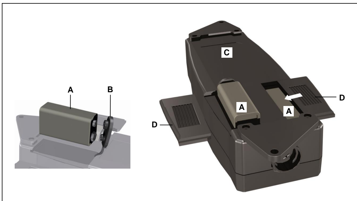
Figure 16 Connecting the batteries
