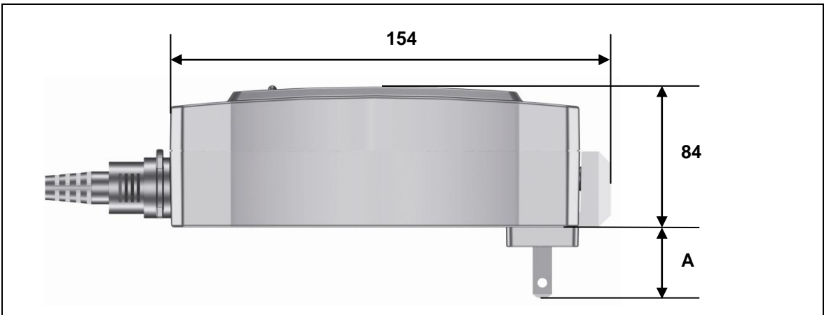
Figure 10 Dimensions of the PD12 POWER SUPPLY (pluggable unit), side view (in mm) A Plug size
