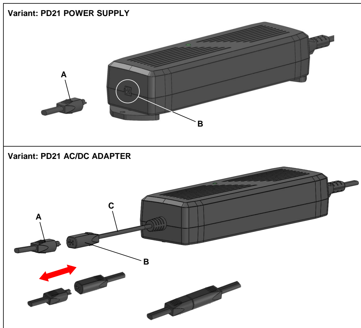
Figure 11 Connection for the drive or control unit
