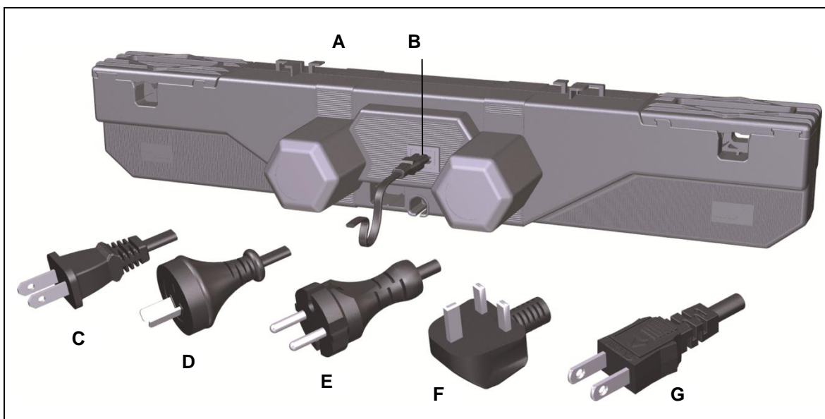
Figure 3 Variants of the power supply cord with the integrated switched-mode power supply (IPS)
