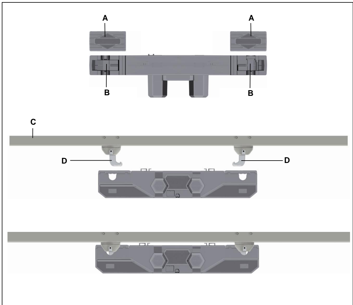
Figure 7 Installing the double drive
