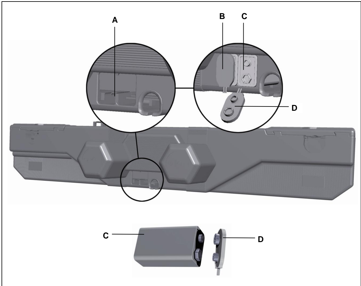
Figure8 Connecting the 9-V batteries
