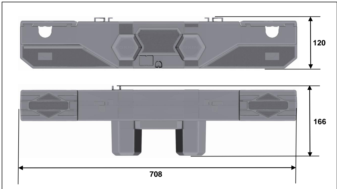
Figure 5 Dimensions of the OKIMAT 2 / OKIMAT 3 drives (in mm)
