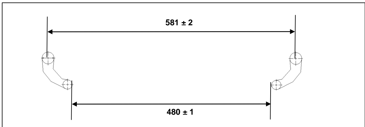
Figure 6 Dimensions of the pivot lever on the brackets (in mm)
