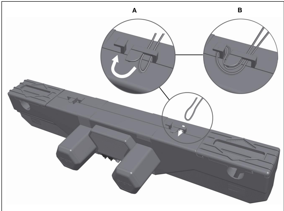
Figure 9 Looping the cable through the strain relief mechanism
